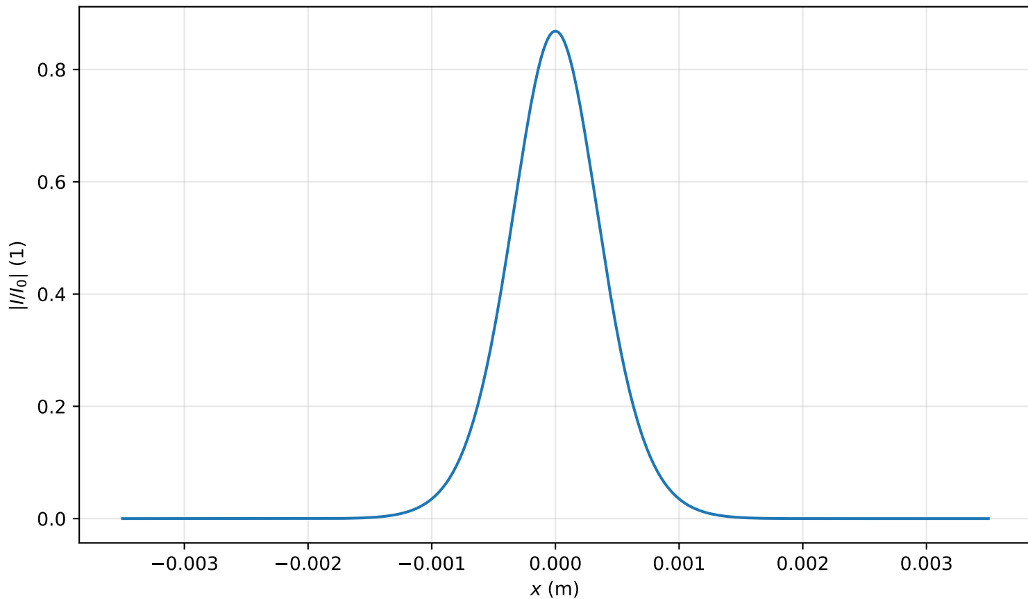
Intensity profile I(x, y = 0, z = 1.513m)/I_0 , P_{in}=0.4P_{cr} , artificial time
